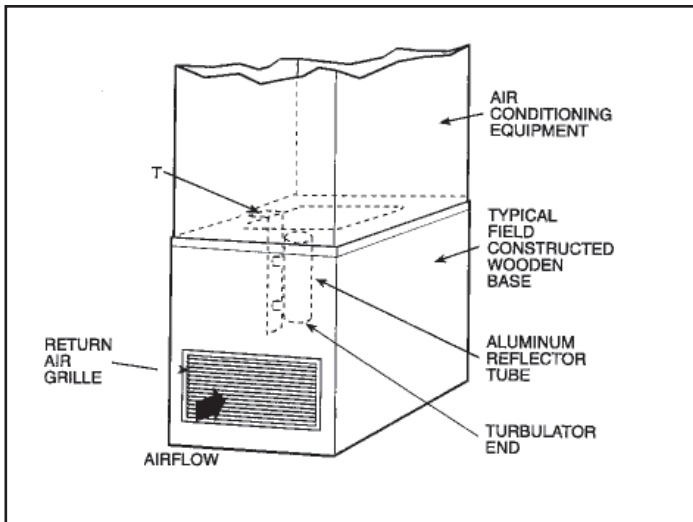
Figure 1. Remote Installation
