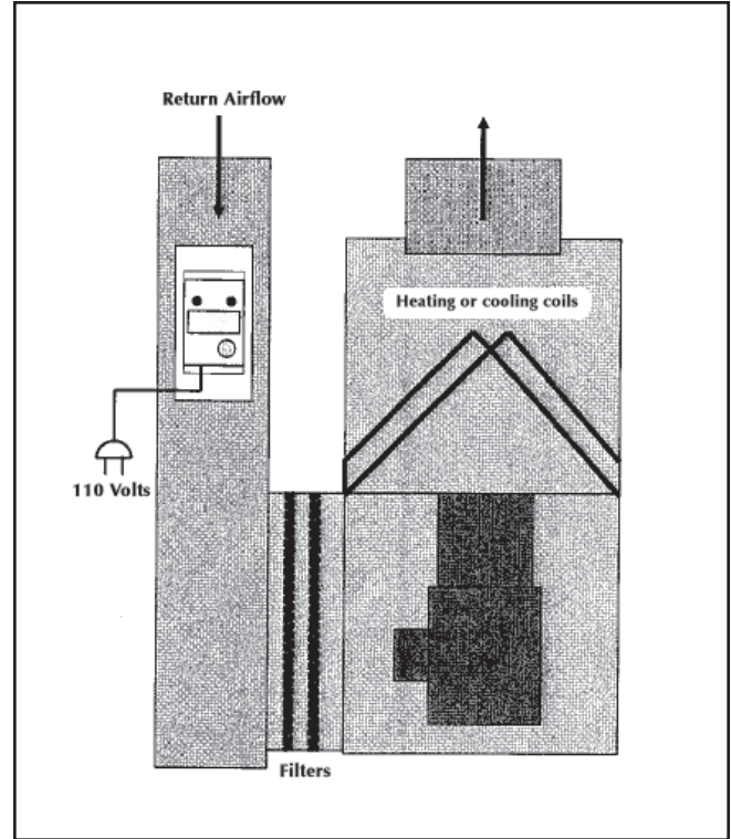
Figure 2. In-Duct Installation
